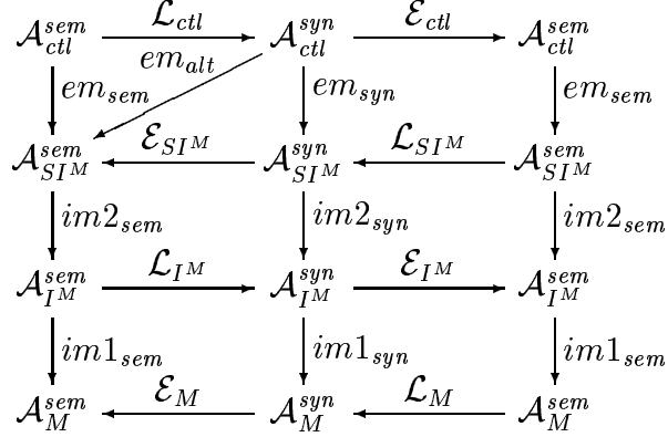
Fig. 6. An algebraic compiler with an imperative specification language layer.
