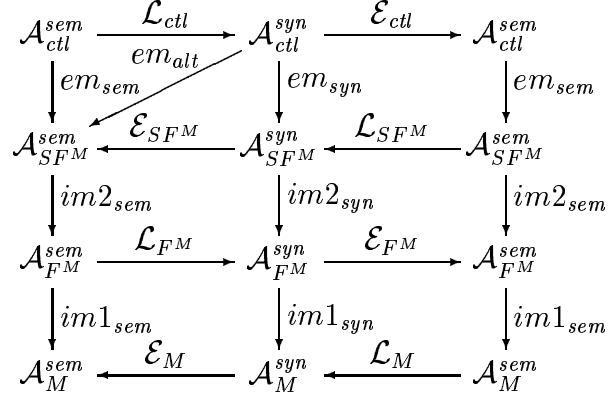
Fig. 5. An algebraic compiler with a functional specification language layer.
